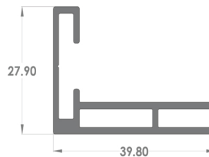
PROFILE DIMENSIONS
